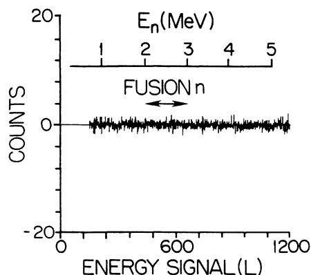
FIG. 4. Net neutron events (cell on - cell off) for a period of 200 h using inverted geometry and cast sample (see Fig. 3).
