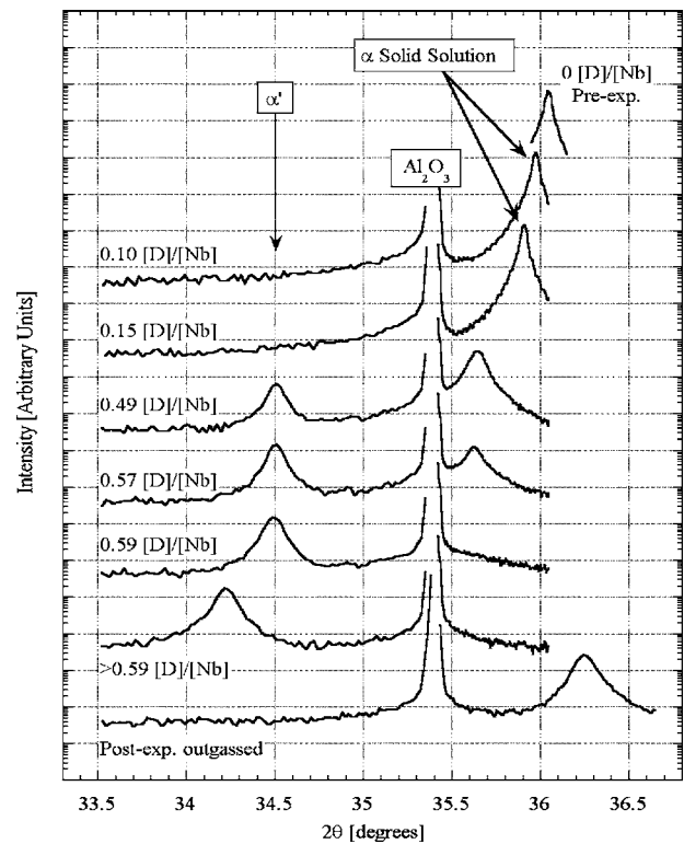
FIG. 3. Second-order specular scans of the 1102 Å film ( \lambda=0.7237 Å) during deuterium gas exposure. Deuterium atomic fraction increases from top to bottom, as labeled. The shift of the ( 2\bar{2}0 ) Nb reflection due to solid solution deuterium absorption is evident, as is discontinuous \alpha \rightarrow \alpha' phase transformation. The post-exposure, post-outgas scan exhibits compressive strain.
